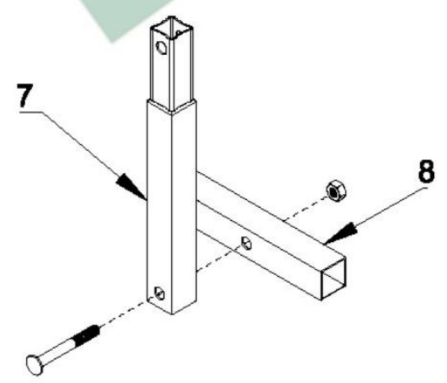
P (1:5)
